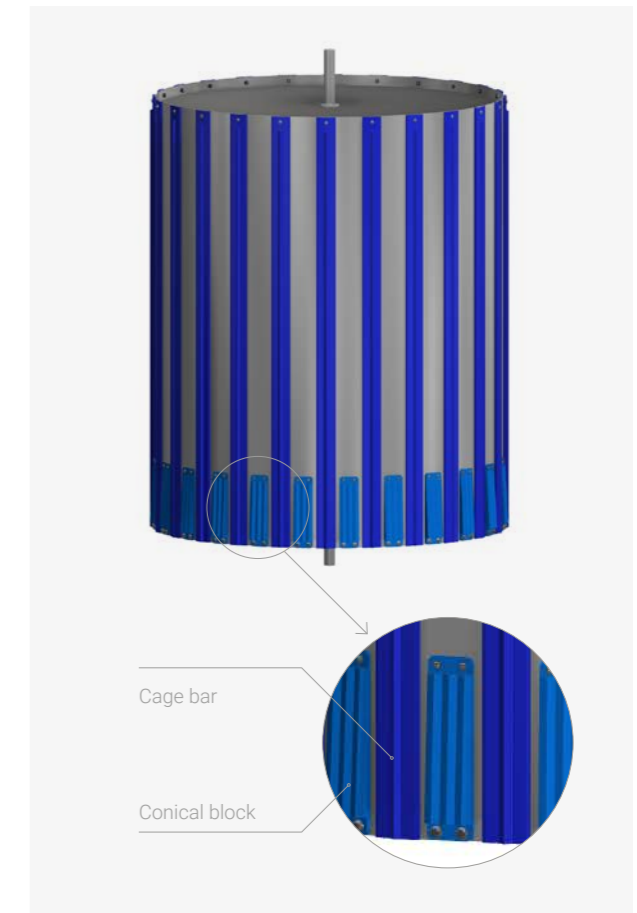
INSIDE DIRECT DRIVE DRUM
