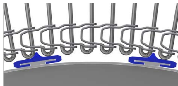
TOP VIEW OF THE CAGE BAR ENGAGING THE BELT
